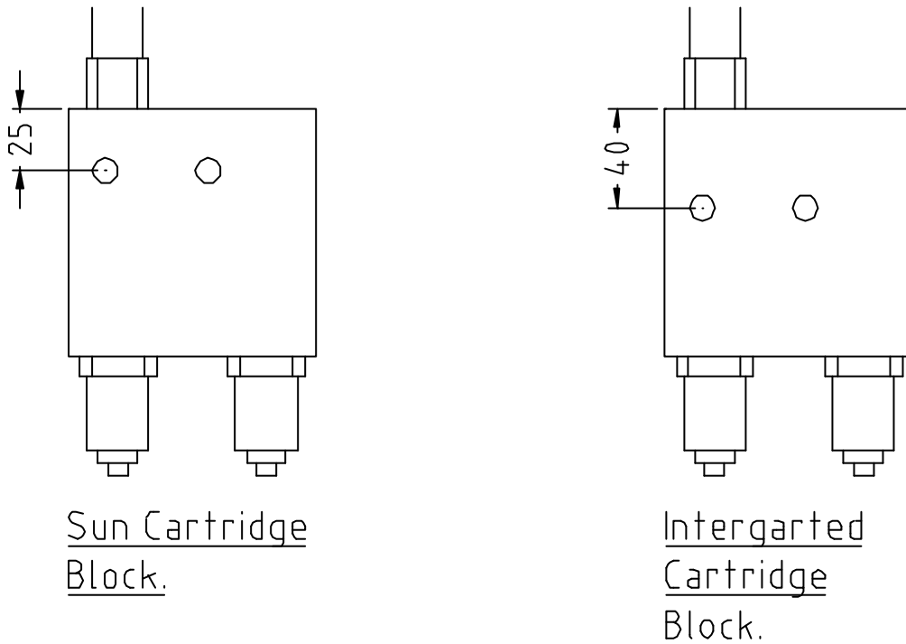
Figure 1.0: Sun and Integrated Hydraulic Cartridge blocks showing the 15mm difference in attaching hole positions.
